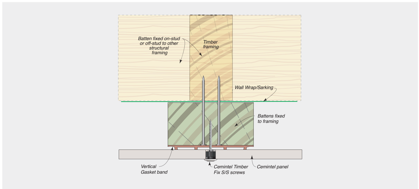
FIGURE 6.01 Panel Fixing at Intermediate Batten
