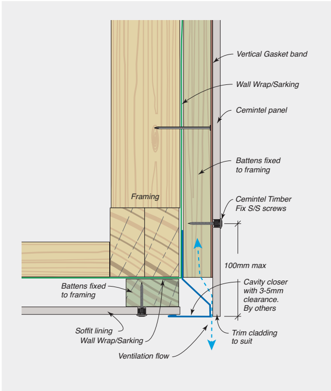
FIGURE 6.10 Soffit Detail
