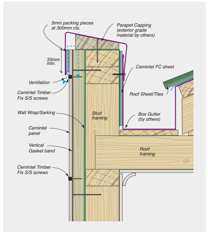
FIGURE 6.14 Parapet Detail
