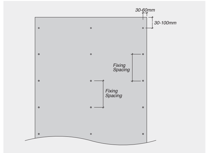
FIGURE 5.02 Vertical Sheet Fixing
