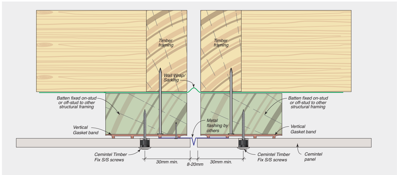
FIGURE 6.03 Panel Fixing At Control Joint
