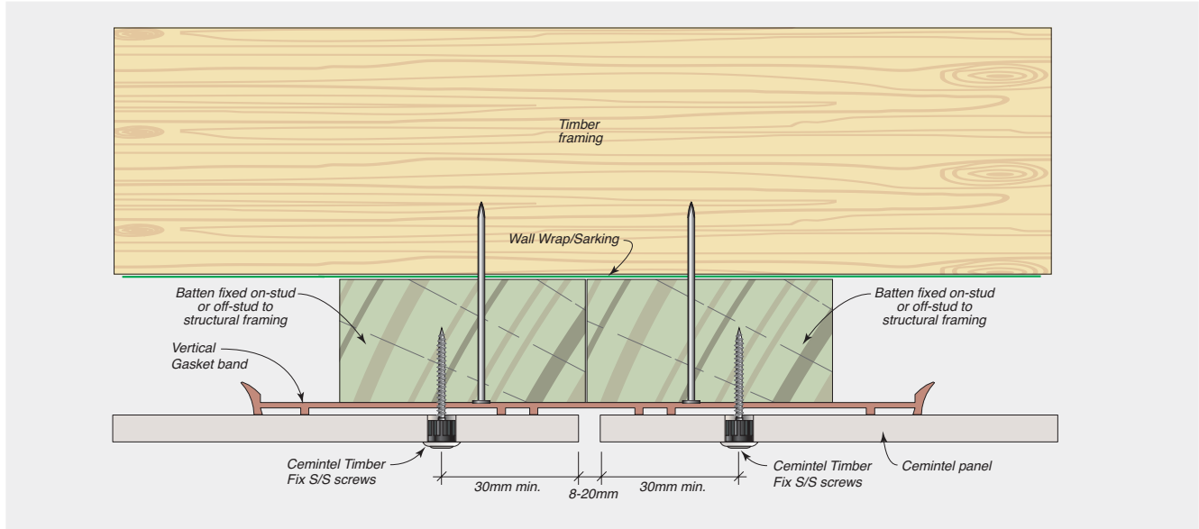
FIGURE 6.02 Panel Fixing At Vertical Joint
