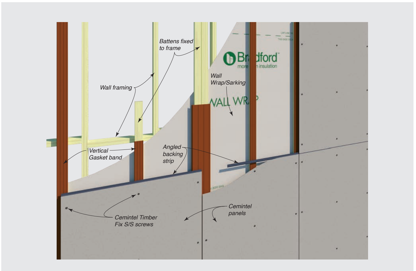
FIGURE 2.01 Barestone External and Surround on Timber Battens Overview
