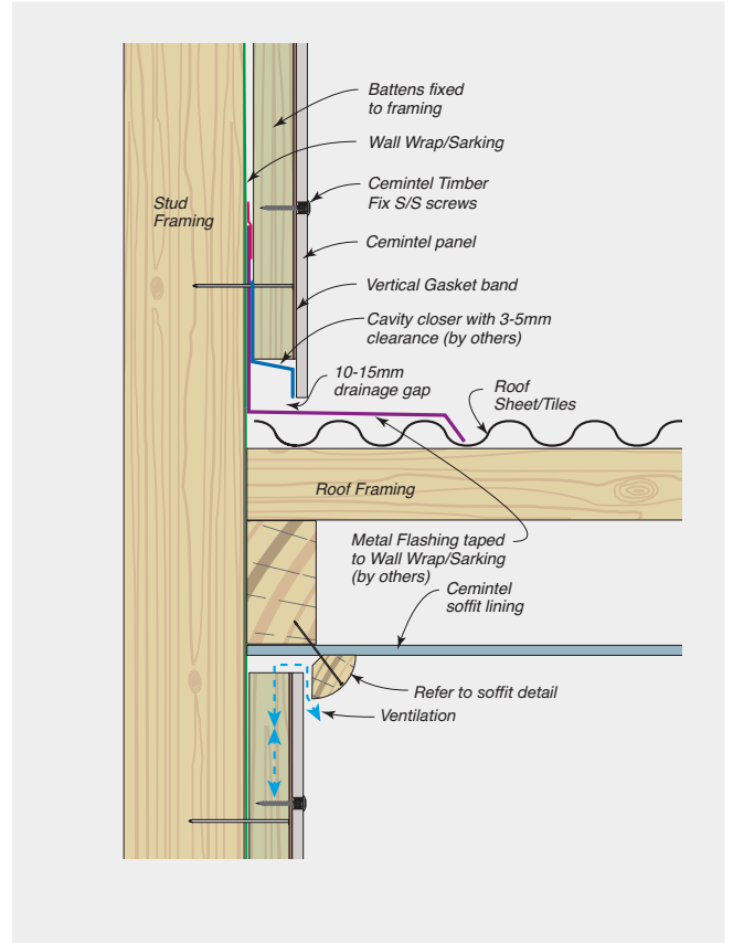
FIGURE 6.13 Raked Roof Intersection
