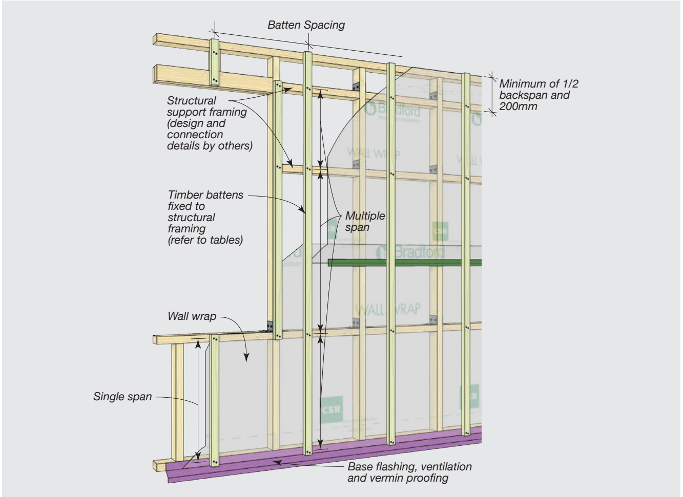
FIGURE 4.01 Battens Off-Stud
