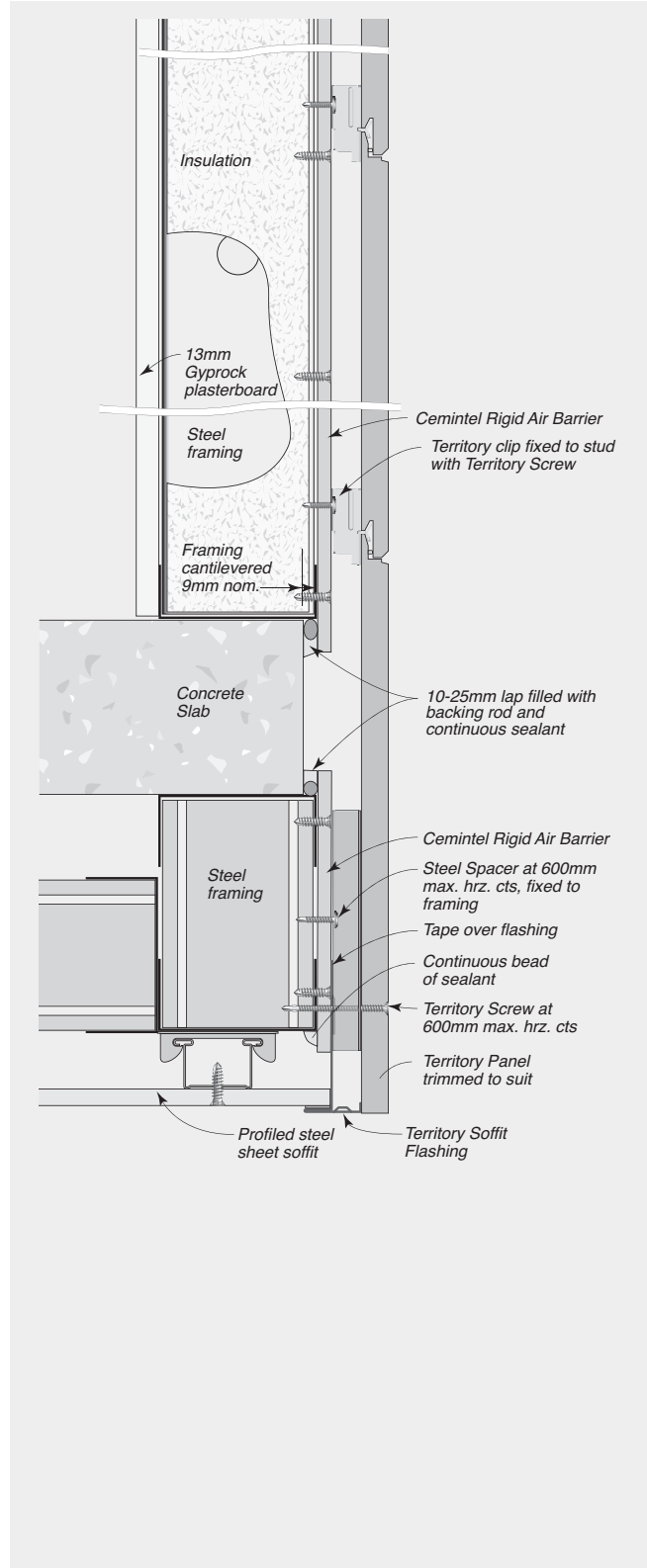
FIGURE 8.64 Metal Ceiling
