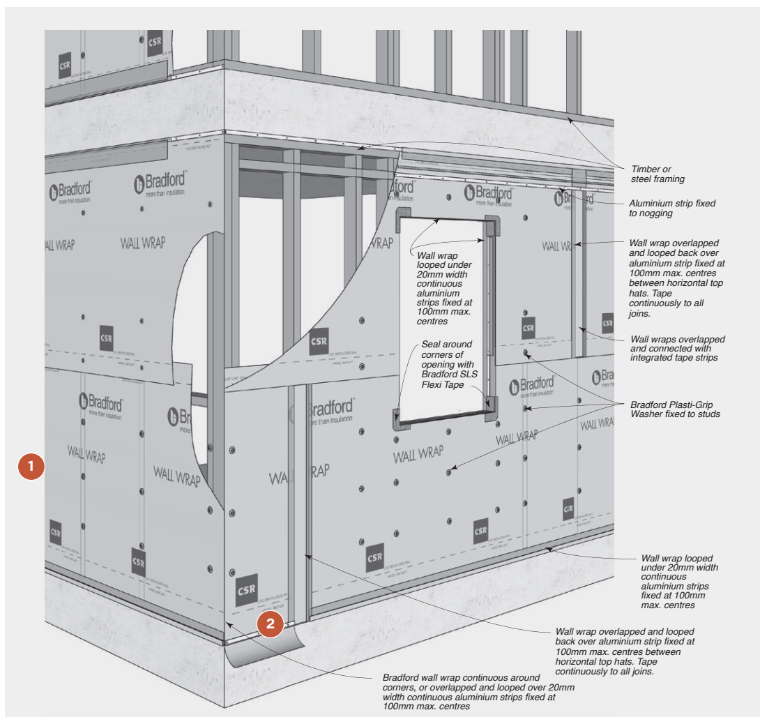
FIGURE 7.03 Typical Soft Air Barrier Installation
