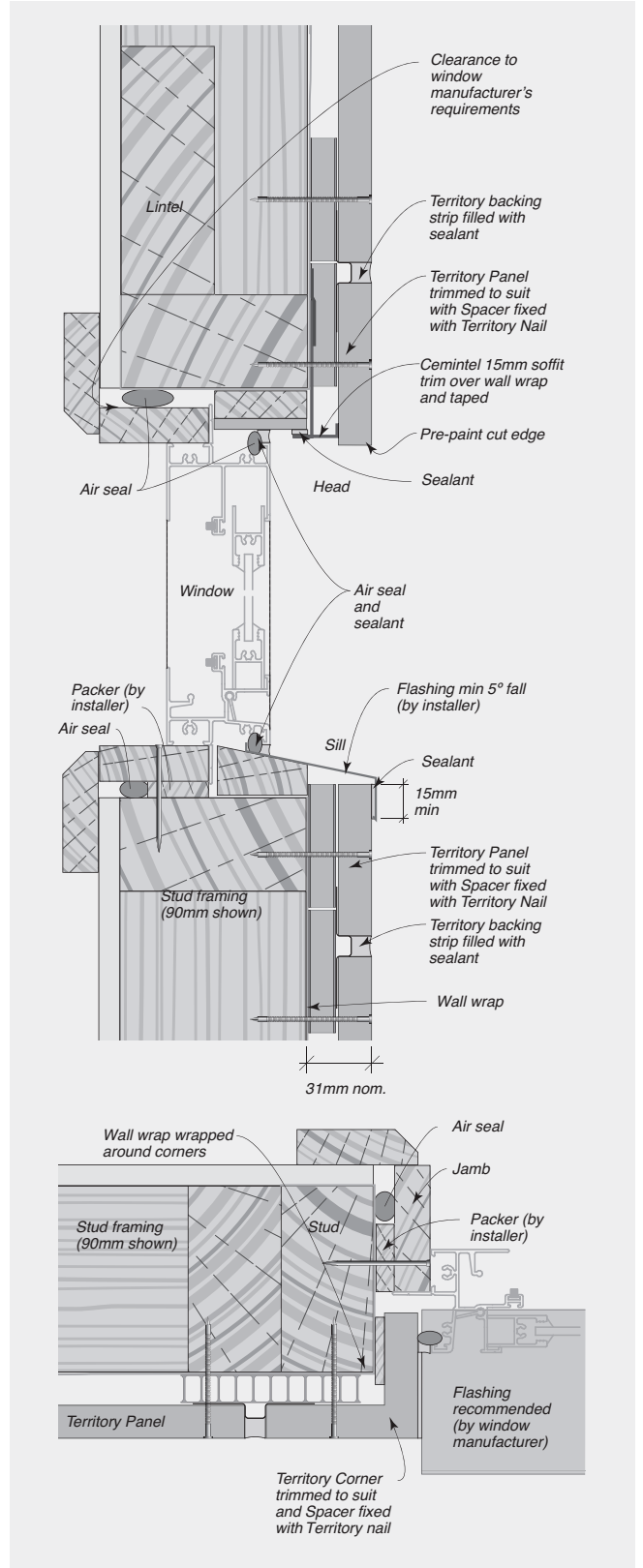
FIGURE 8.29 Window Reveal
