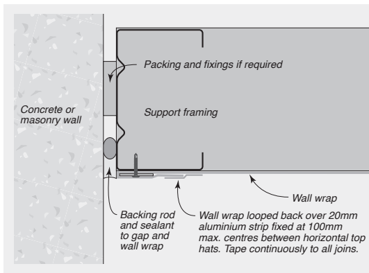
FIGURE 8.73 Abutment to Concrete or Masonry Wall
