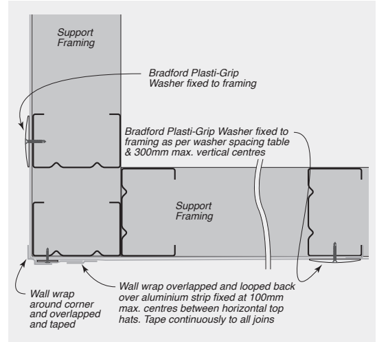
FIGURE 8.71 External Corner – Wall Wrap Overlapped
