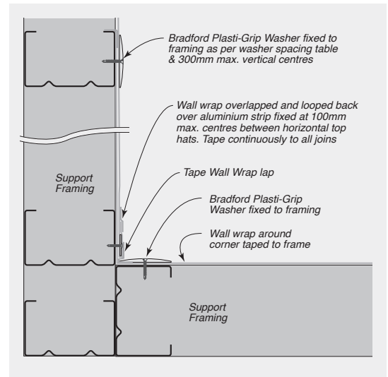
FIGURE 8.74 Internal Corner – Wall Wrap Overlapped
