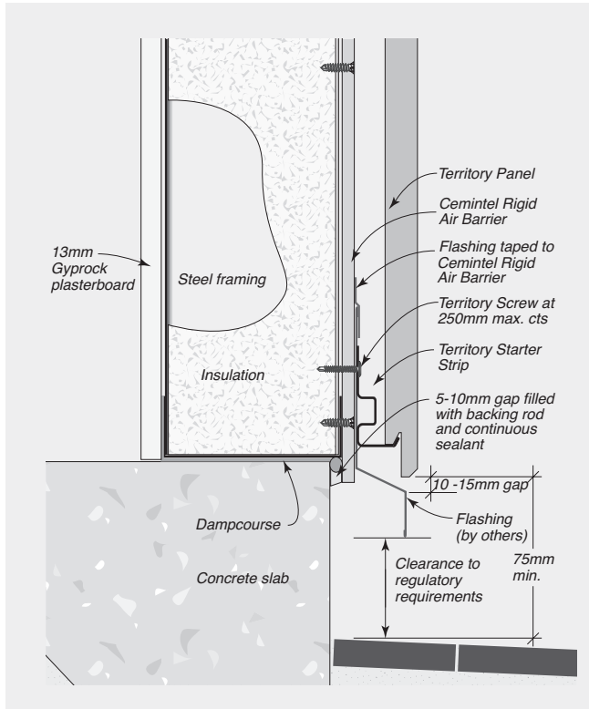
FIGURE 8.53 Base Detail
