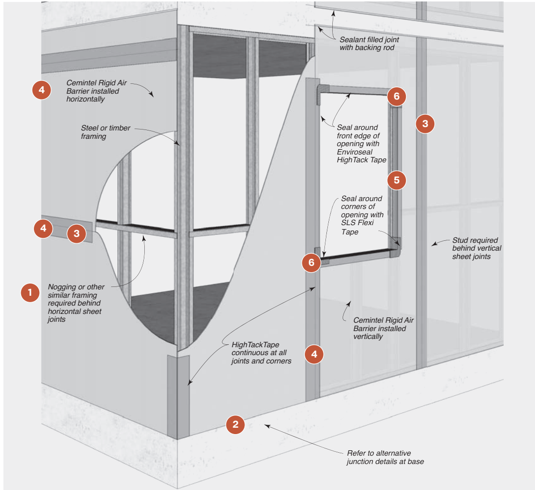
FIGURE 7.01 Typical Rigid Air Barrier Installation
