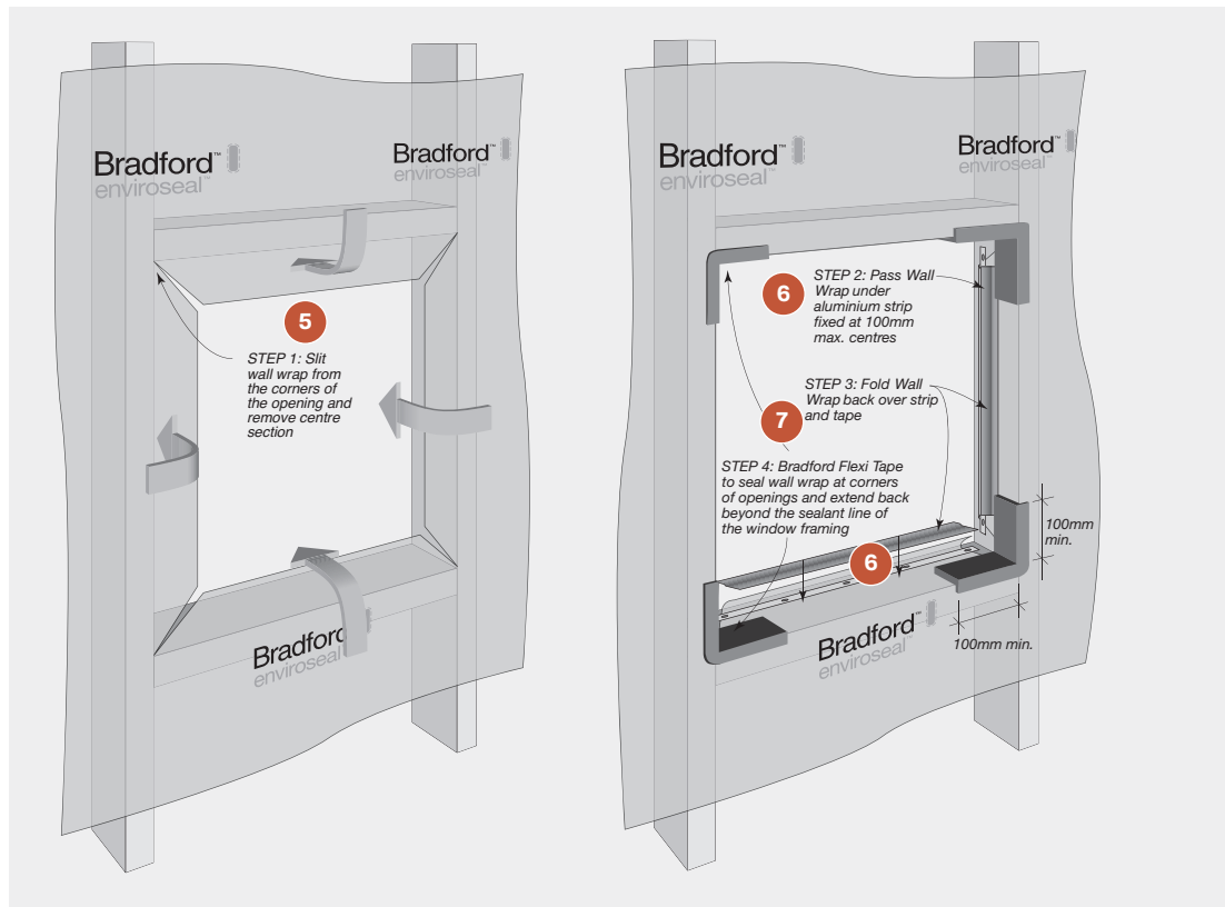
FIGURE 7.04 Treatment at Window/Door Openings - Soft Air Barrier
