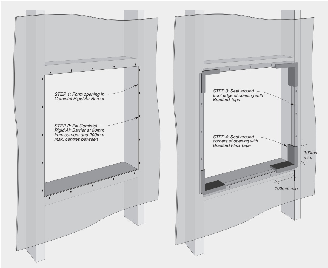
FIGURE 7.02 Treatment at Window/Door Openings - Rigid Air Barrier
