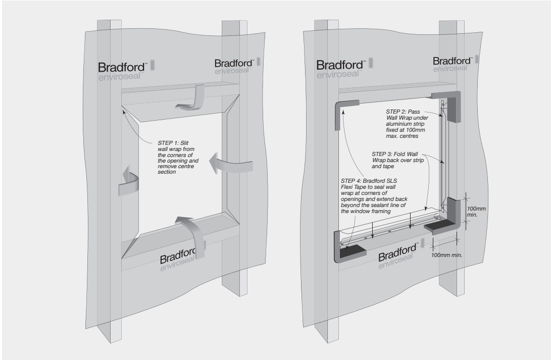
FIGURE 8.82 Wall Wrap Installation at Window/Door Opening
