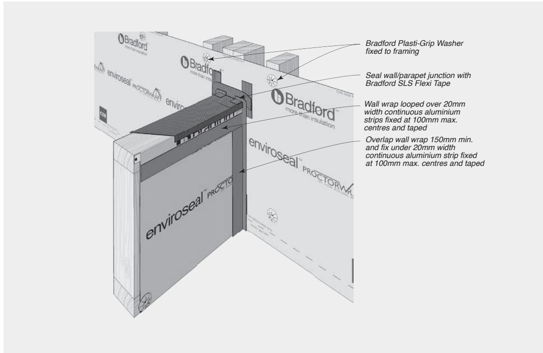
FIGURE 8.83 Wall Wrap Installation at Parapet Junction – Timber or Steel Framing
