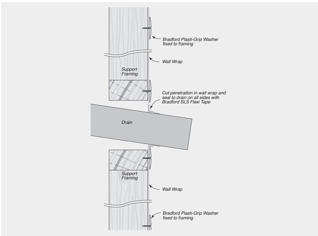
FIGURE 8.81 Wall Wrap Installation at Drain Penetration – Timber or Steel Framing
