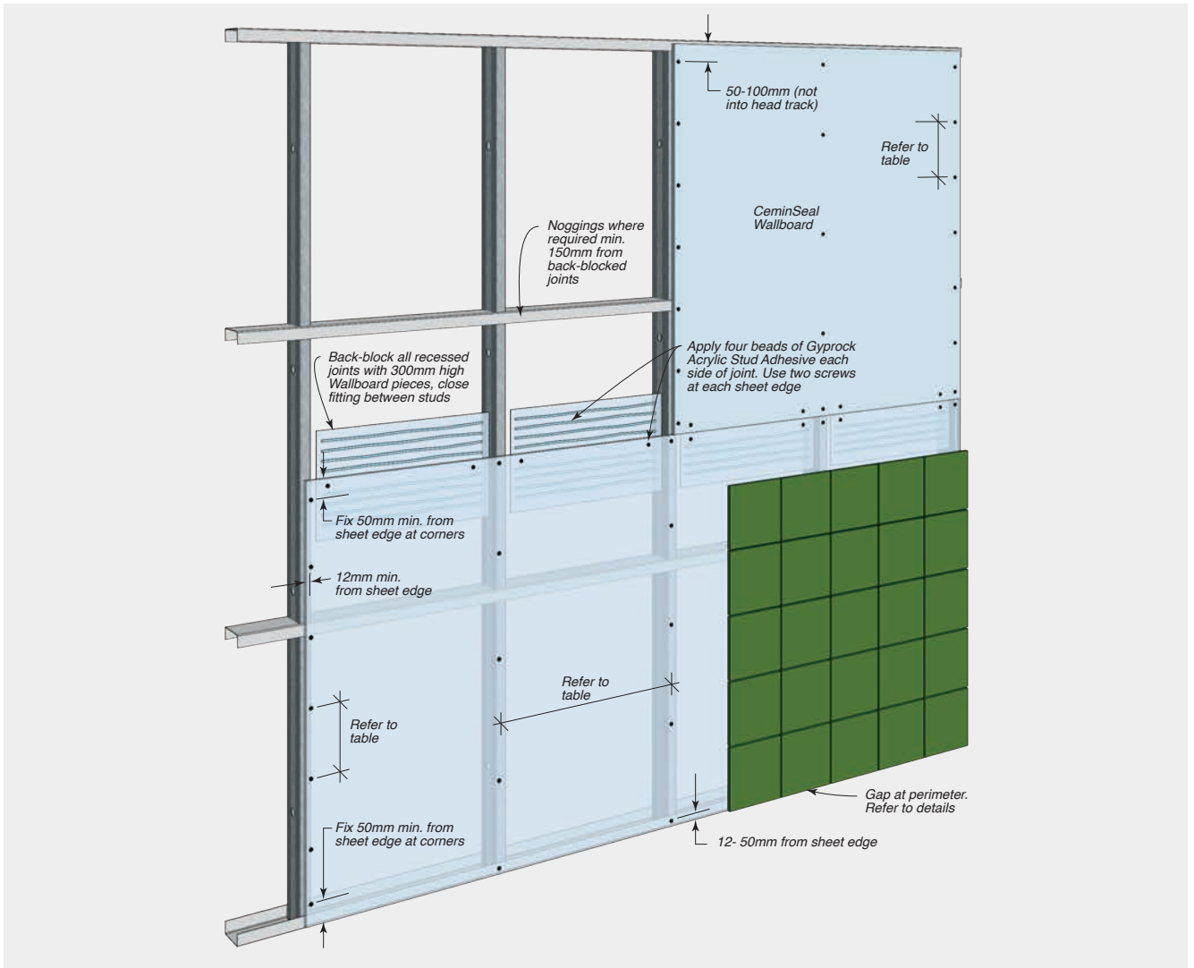
FIGURE 8.06 CeminSeal Wallboard Fixing To Stud Framing – Horizontal Sheeting With Back-Blocked Joints – Fastener Fixing – Non-Tiled Or Tiled Areas (Alternative Installation)
