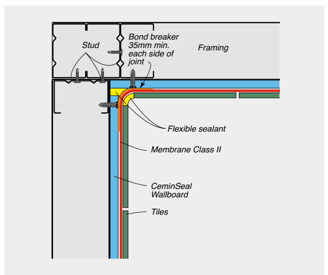
FIGURE 9.22 Internal Corner Detail – Class II Membrane (Provide back blocking or non-ferrous angle to studs to prevent differential movement.)
