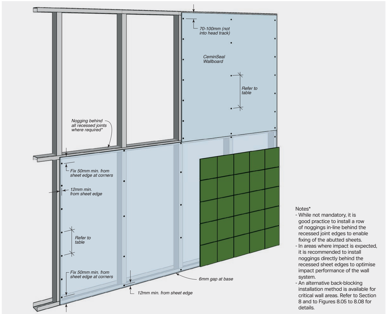
FIGURE 7.02 Ceminseal Wallboard Fixing To Stud Framing – Horizontal Sheeting – Fastener Fixing – Non-tiled Or Tiled Areas
