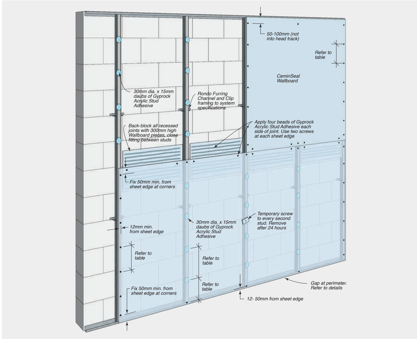
FIGURE 8.07 CeminSeal Wallboard Fixing To Furring Channel Framing – Horizontal Sheeting With Back-Blocked Joints – Adhesive + Fastener Fixing – Non-Tiled Areas (Alternative Installation)
