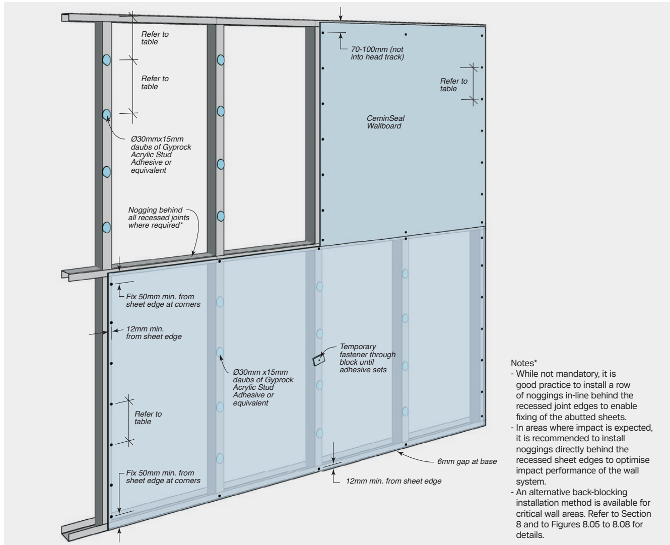
FIGURE 7.01 Ceminseal Wallboard Fixing To Stud Framing – Horizontal Sheeting – Adhesive + Fastener Fixing – Non-Tiled Areas
