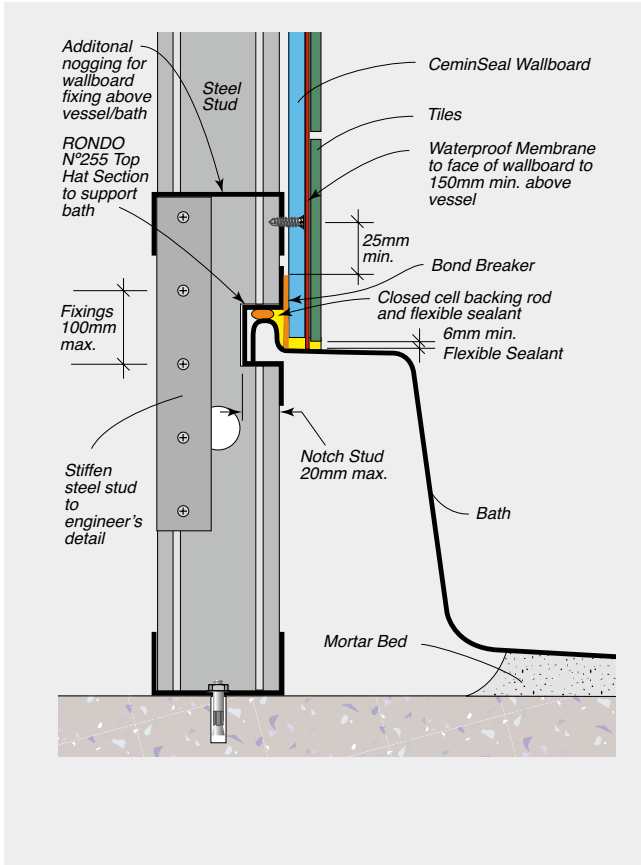
FIGURE 9.26 Bath Installation To Stud Wall
