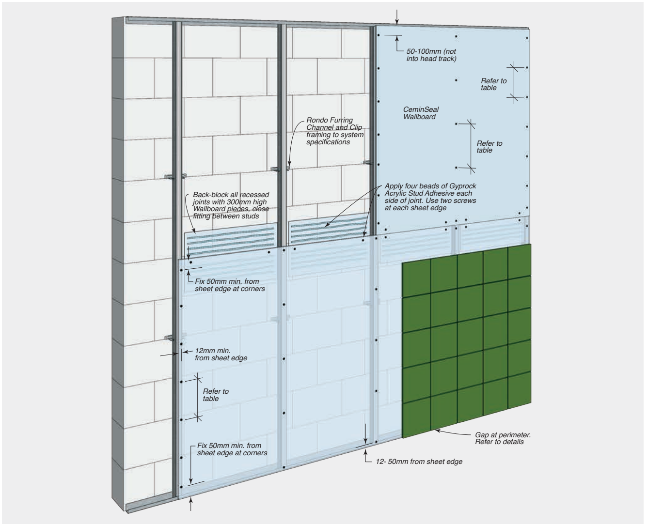
FIGURE 8.08 CeminSeal Wallboard Fixing To Furring Channel Framing – Horizontal Sheeting With Back-Blocked Joints – Fastener Fixing – Non-Tiled Or Tiled Areas (Alternative Installation)
