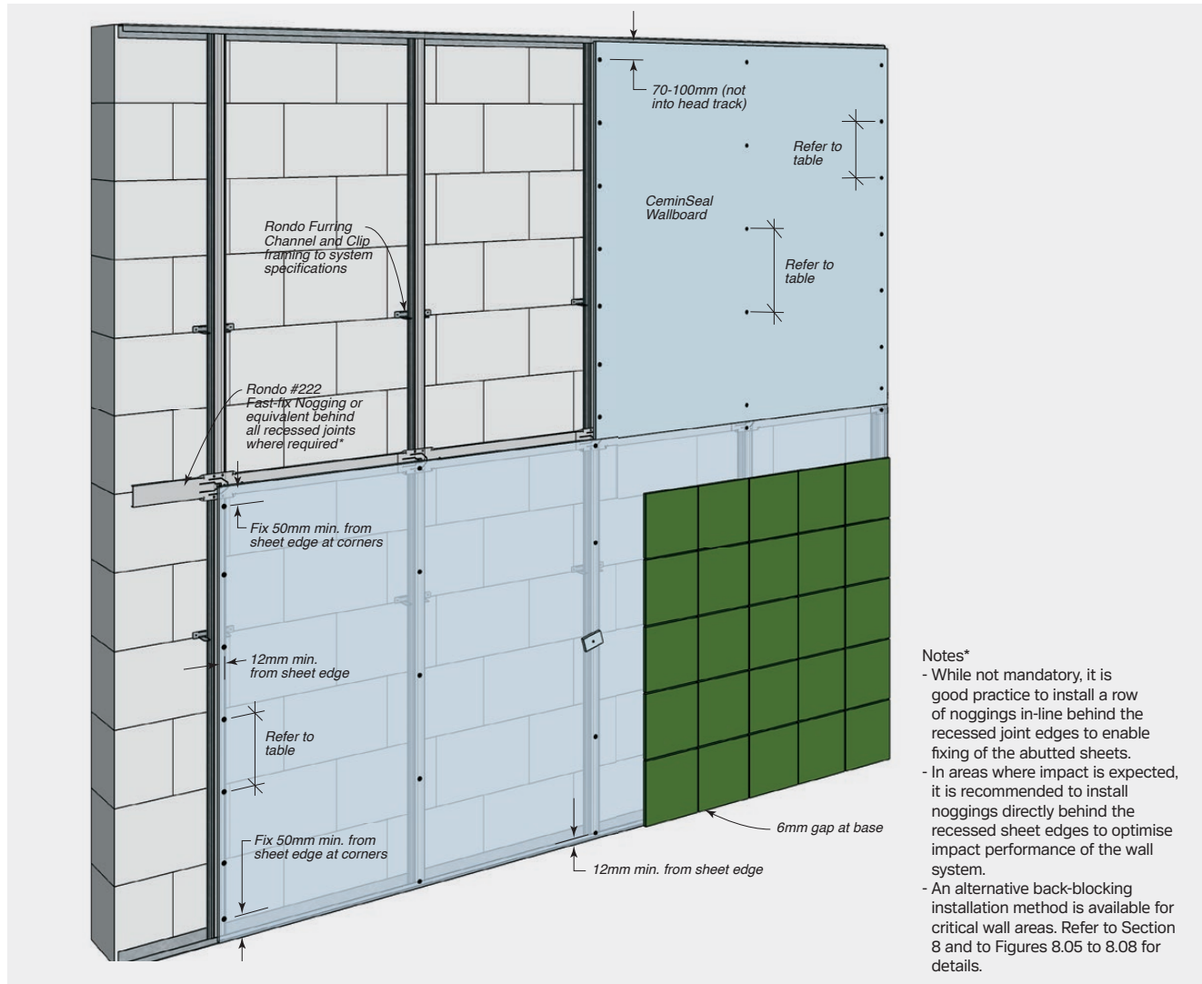
FIGURE 7.05 Ceminseal Wallboard Fixing To Furring Channel Framing – Horizontal Sheeting – Fastener Fixing – Non-Tiled Or Tiled Areas
