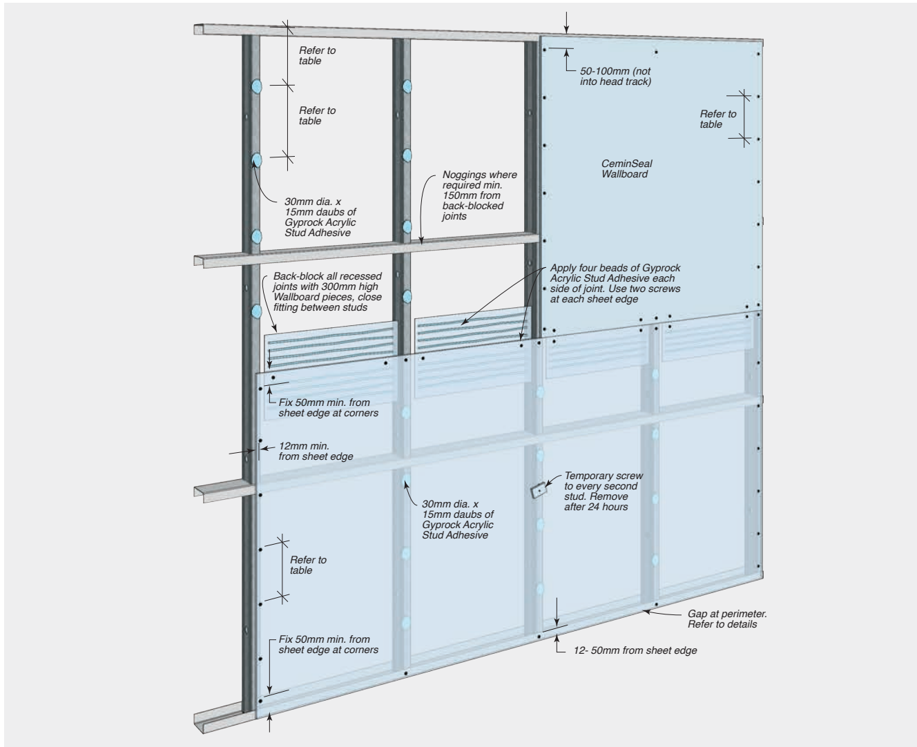
FIGURE 8.05 CeminSeal Wallboard Fixing To Stud Framing – Horizontal Sheeting With Back-Blocked Joints – Adhesive + Fastener Fixing – Non-Tiled Areas (Alternative Installation)
