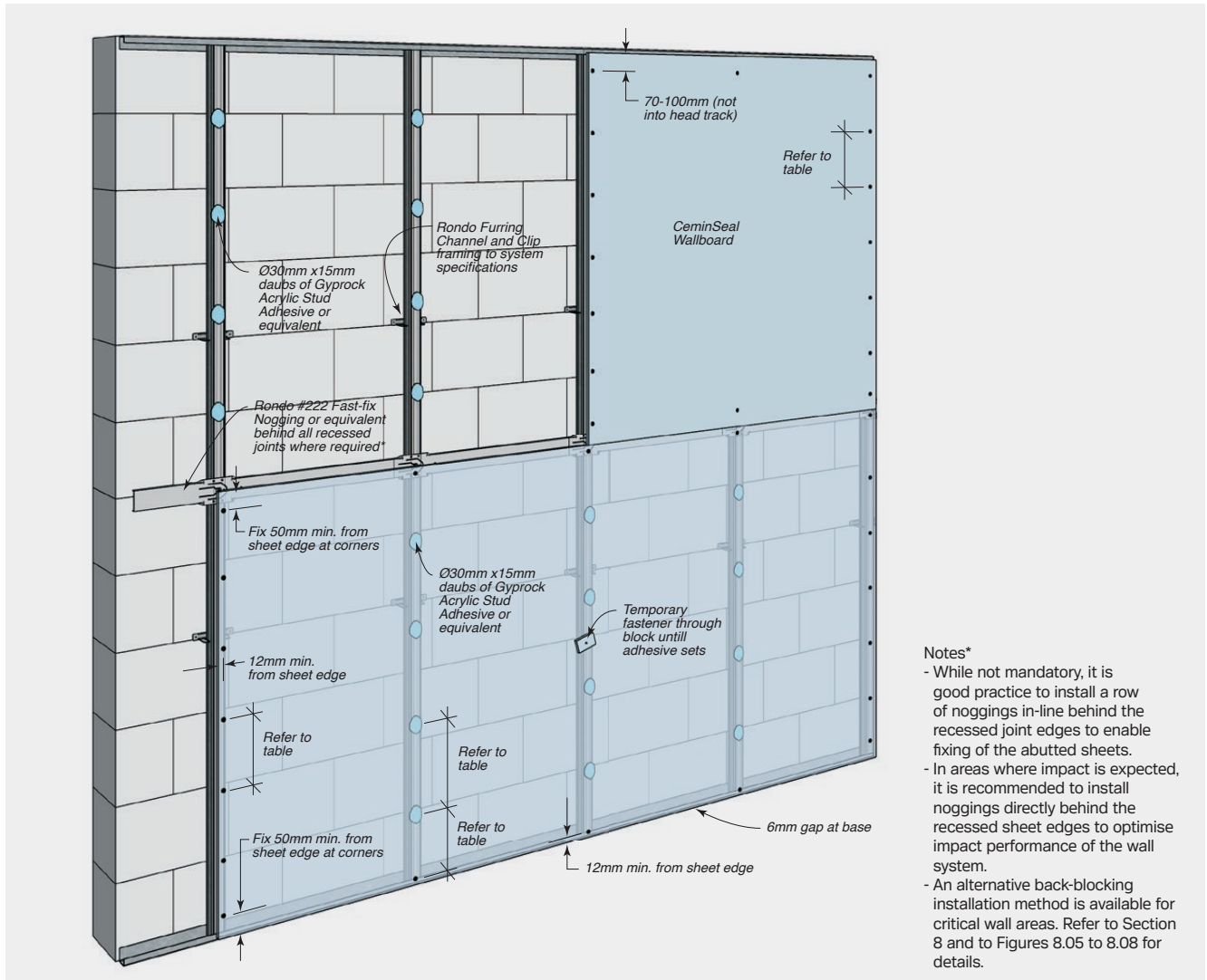
FIGURE 7.04 Cemintel Wallboard Fixing To Furring Channel Framing – Horizontal Sheeting – Adhesive + Fastener Fixing – Non-Tiled Areas
